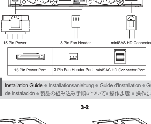
15 Pin Power 3 Pin Fan Header miniSAS HD Connector
